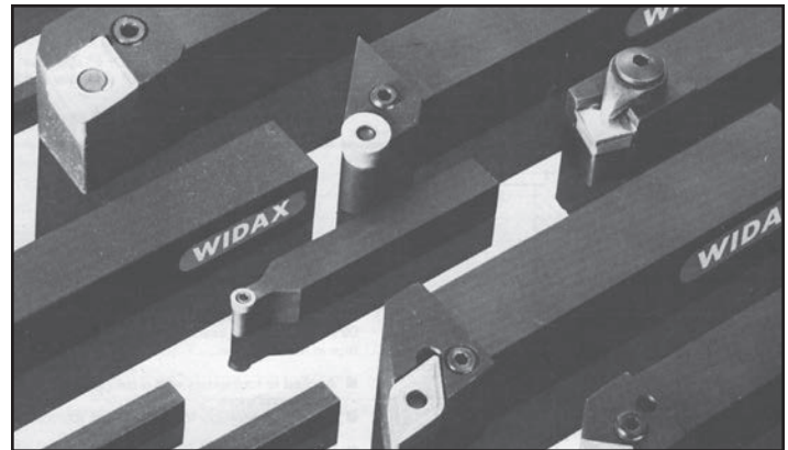
Metric Clamp Lock Toolholders
